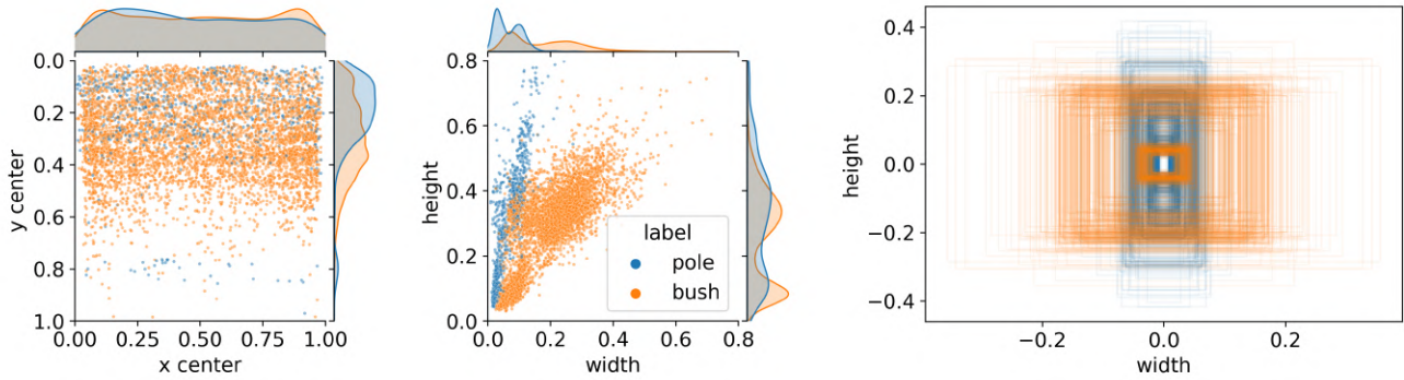
Figure 6. Label statistics: distribution of positions and bounding box dimensions, as well as shape summary (axes are normalized)
